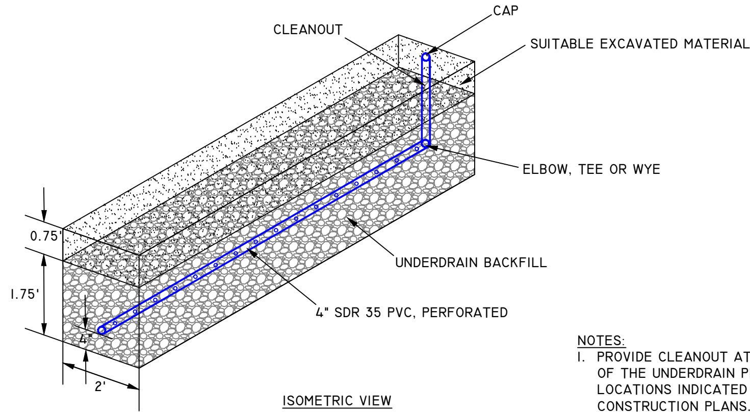
ISOMETRIC VIEW NOT TO SCALE
