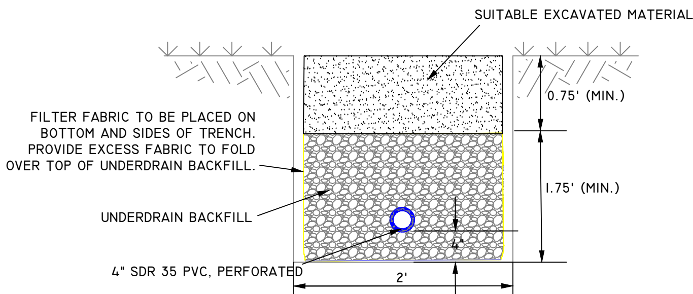
SECTION VIEW NOT TO SCALE
