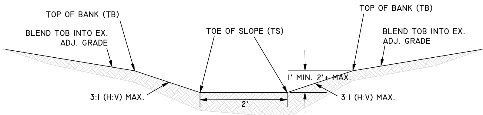
SECTION VIEW NOT TO SCALE
